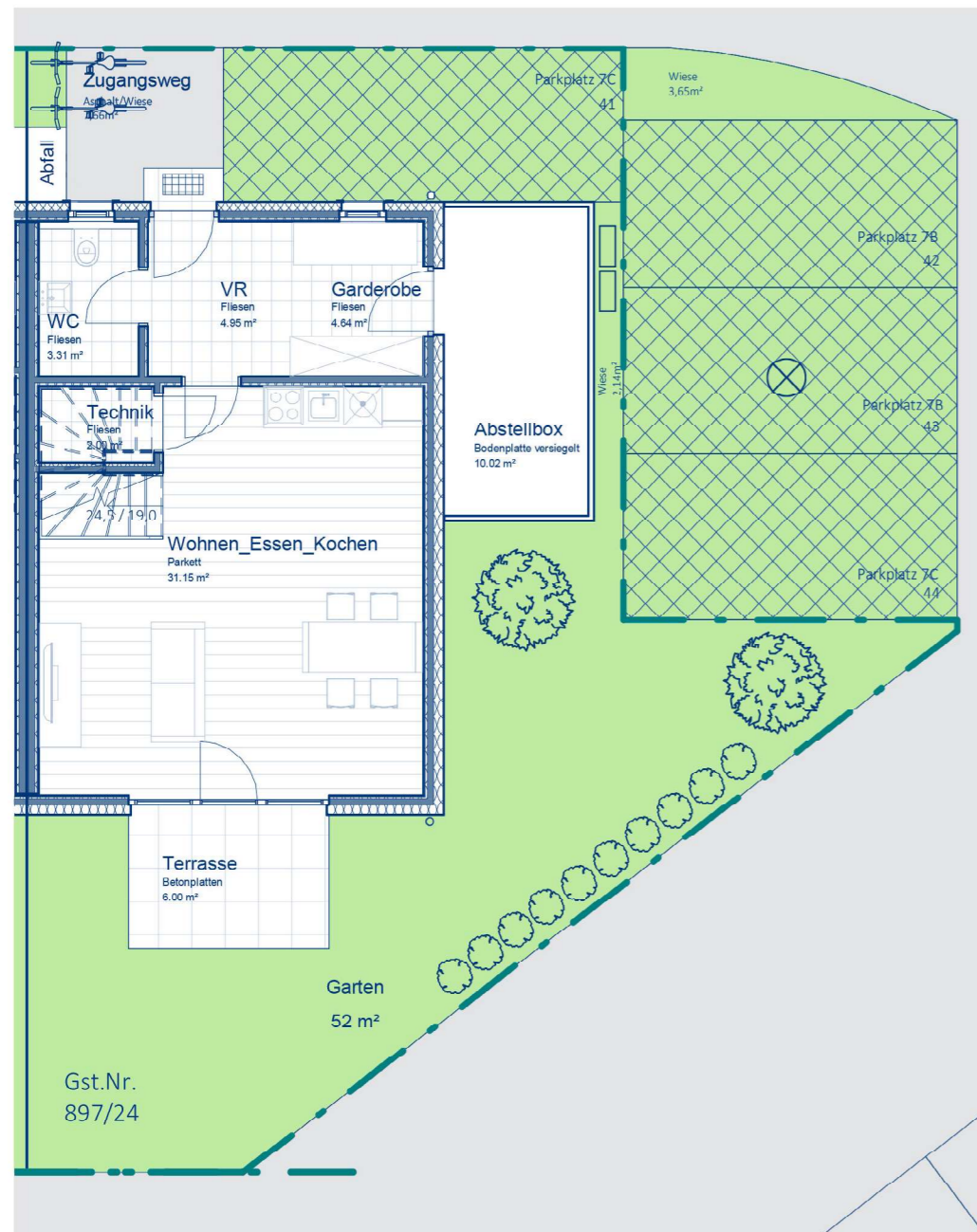
1m Erdgeschoß
